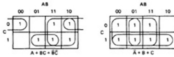
Figure 6.8: KV Charts for Functions of Three Variables.
