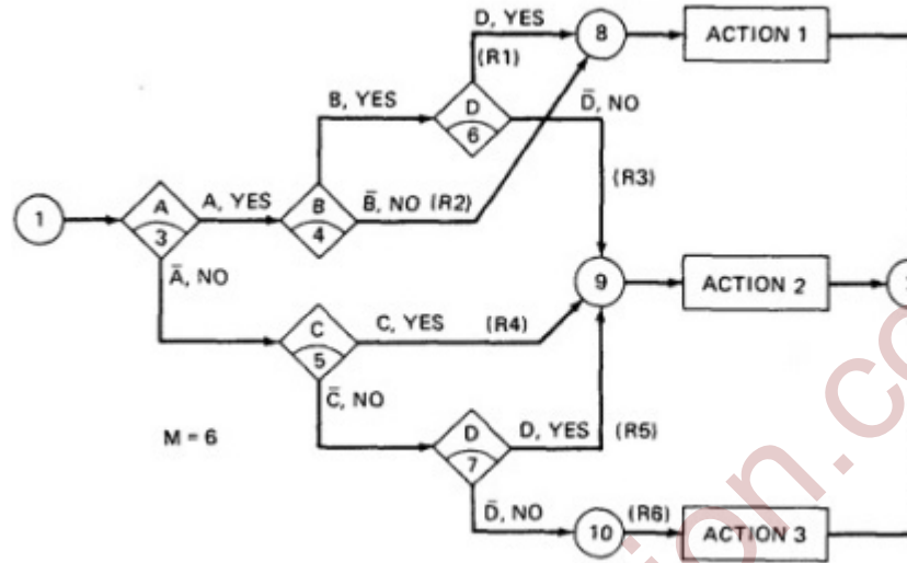
Figure 6.4 : A Sample Program
