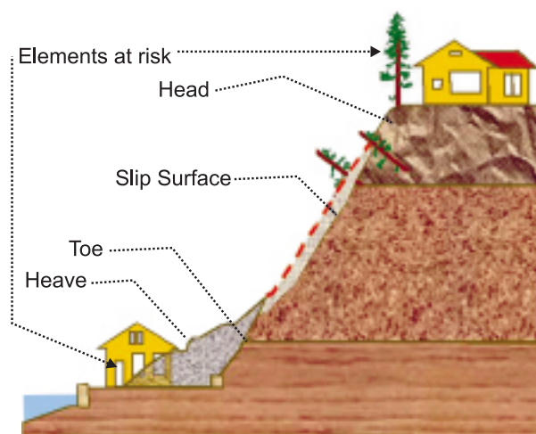
Fig 2.6.4 adverse effects of landslide
