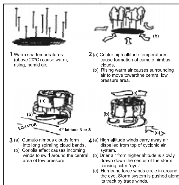
Fig 2.3.2 Stages of cyclone formation
