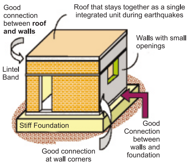
Essential requirements in a Masonry building
